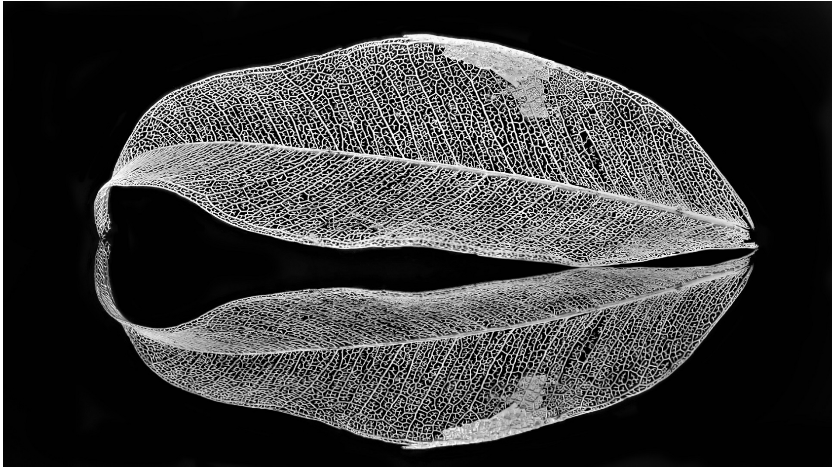
Skeleton Leaf 9971
